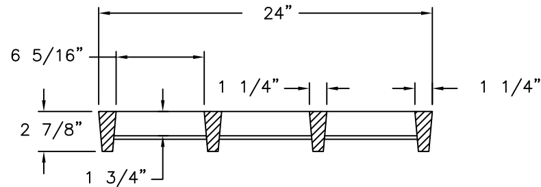
GRATE SECTION
