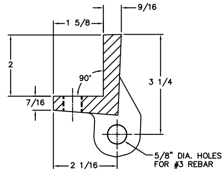
FRAME SECTION
