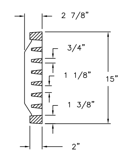
GRATE SECTION
