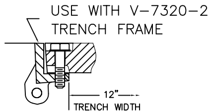
BOLT DOWN DETAIL
